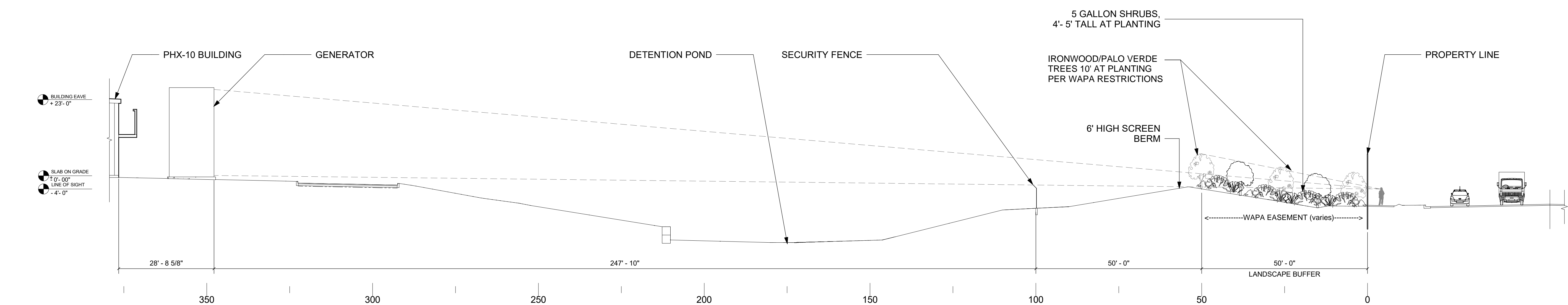
2 EAST - STANDING ON PROPERTY LINE LOOKING WEST 1" = 10'-0"
