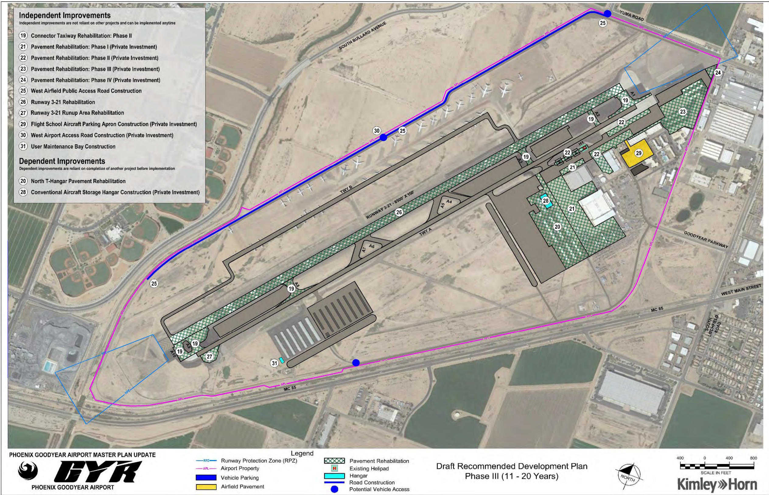
Figure 7-4 Recommended Development Plan: Phase III
