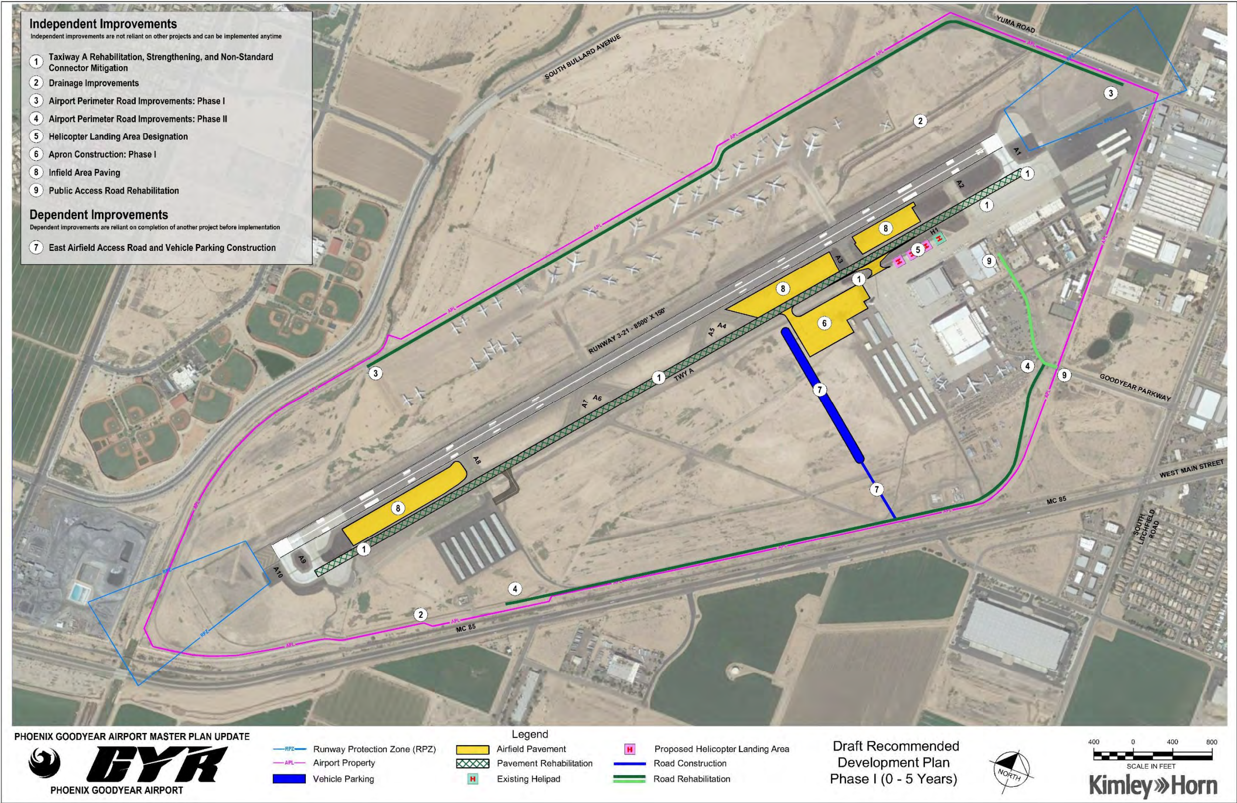
Figure 7-2 Recommended Development Plan: Phase I
