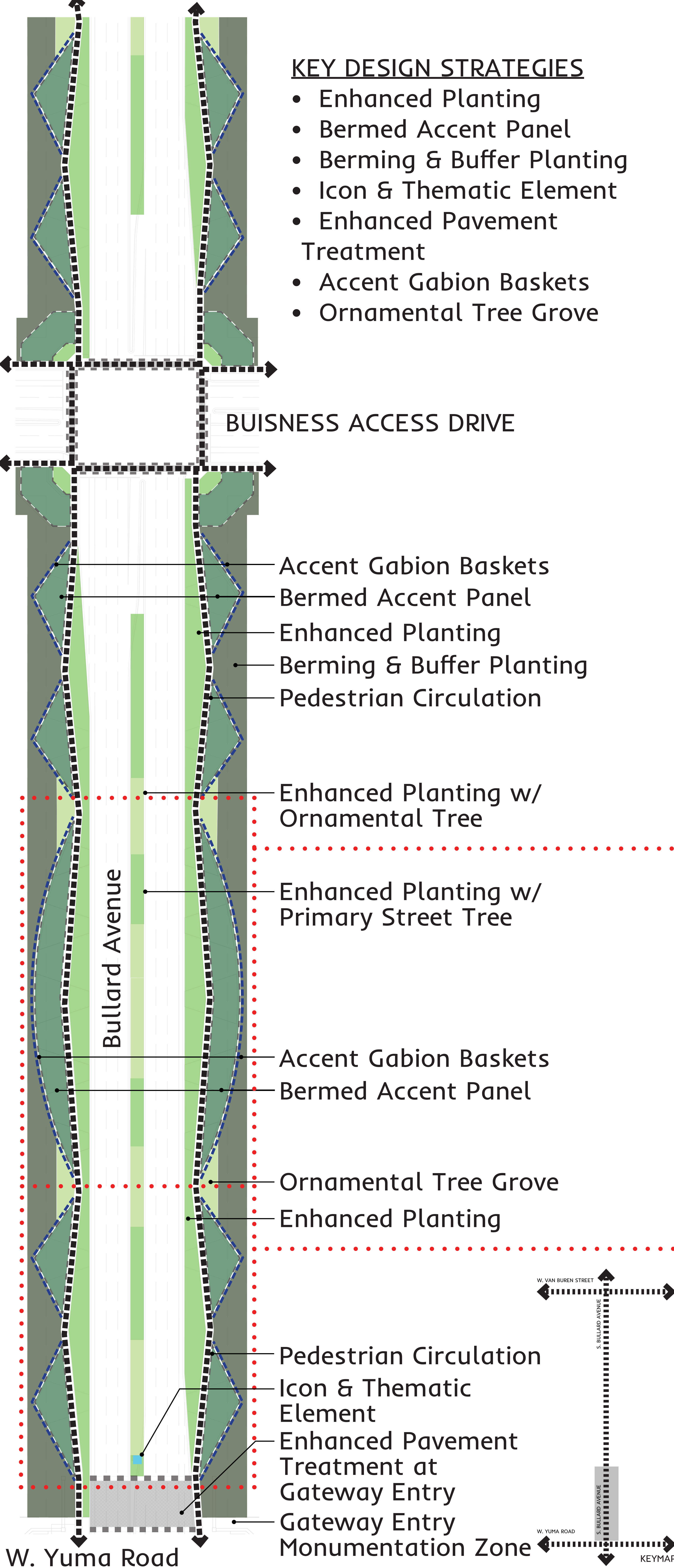
STREETSCAPE ZONE - W. Yuma Road to 1/2 Mile DESIGN FRAMEWORK
